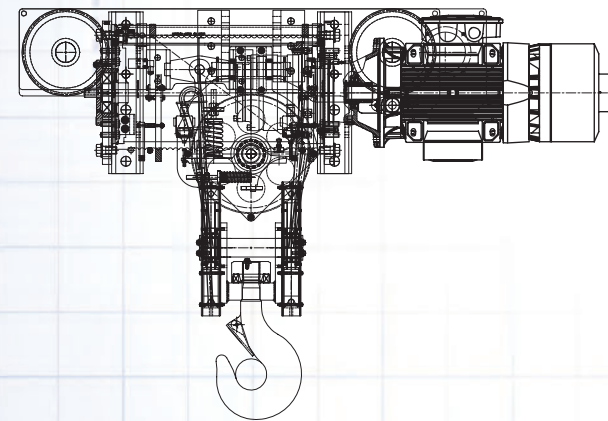
TYPE 26 Top Running Trolley; Single Reeved CAPACITY: 3 – 90 Ton
