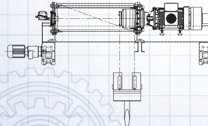
TYPE 26 Top Running Trolley; Single Reeved CAPACITY: 3 – 90 Ton
