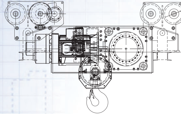
TYPE 23 Monorail Standard Trolley; Single Reeved CAPACITY: 3 – 20 Ton
