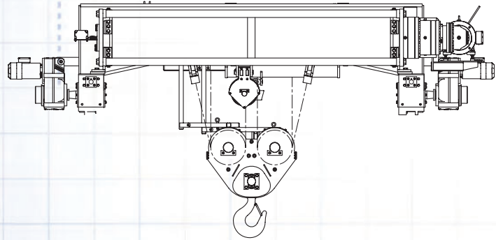
TYPE 19 Top Running Trolley; 2 Part Double Reeving; Double Reeved CAPACITY: 5 – 15 Ton
