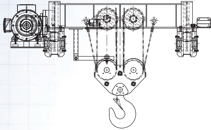
TYPE 18 Top Running Trolley; Standard Profile; Double Reeved CAPACITY: 15 – 160 Ton
